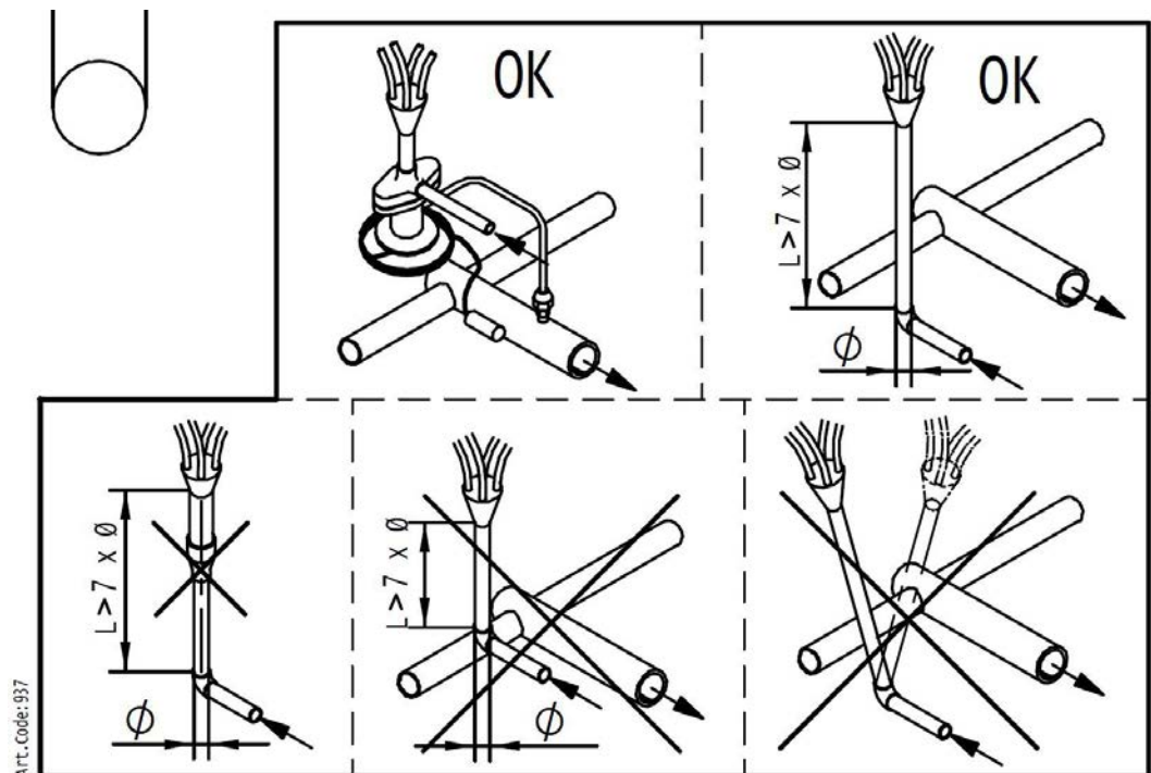
937 - Montage Expansionsventil
