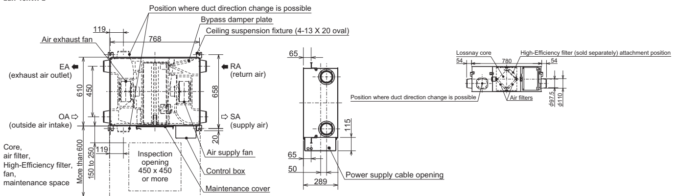
LGH-15RVX-E
