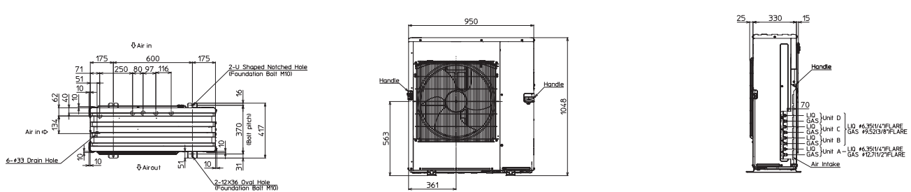
MXZ-4F83VFHZ
