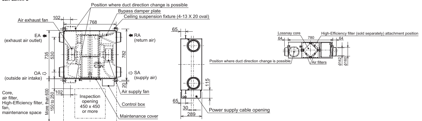
LGH-25RVX-E
