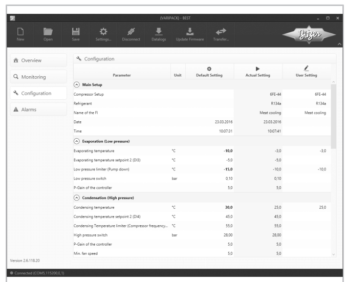
Fig. 22: VARIPACK configuration "Pressure control"
